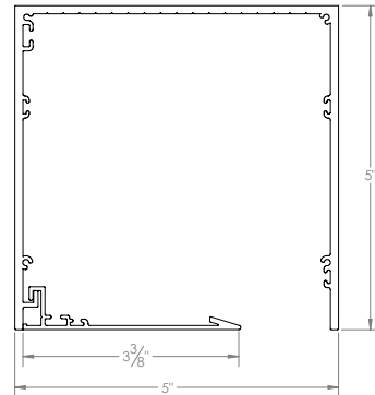
5" POCKET WITH 3 3/8" CLOSURE
